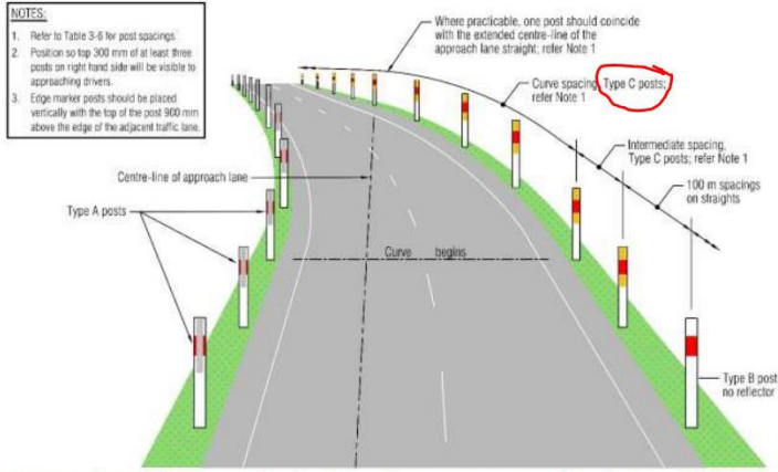
Figure 3-7: Edge marker post installation on all rural state highways and other rural roads with AADT greater than 1,500 vpd – Left hand curve
